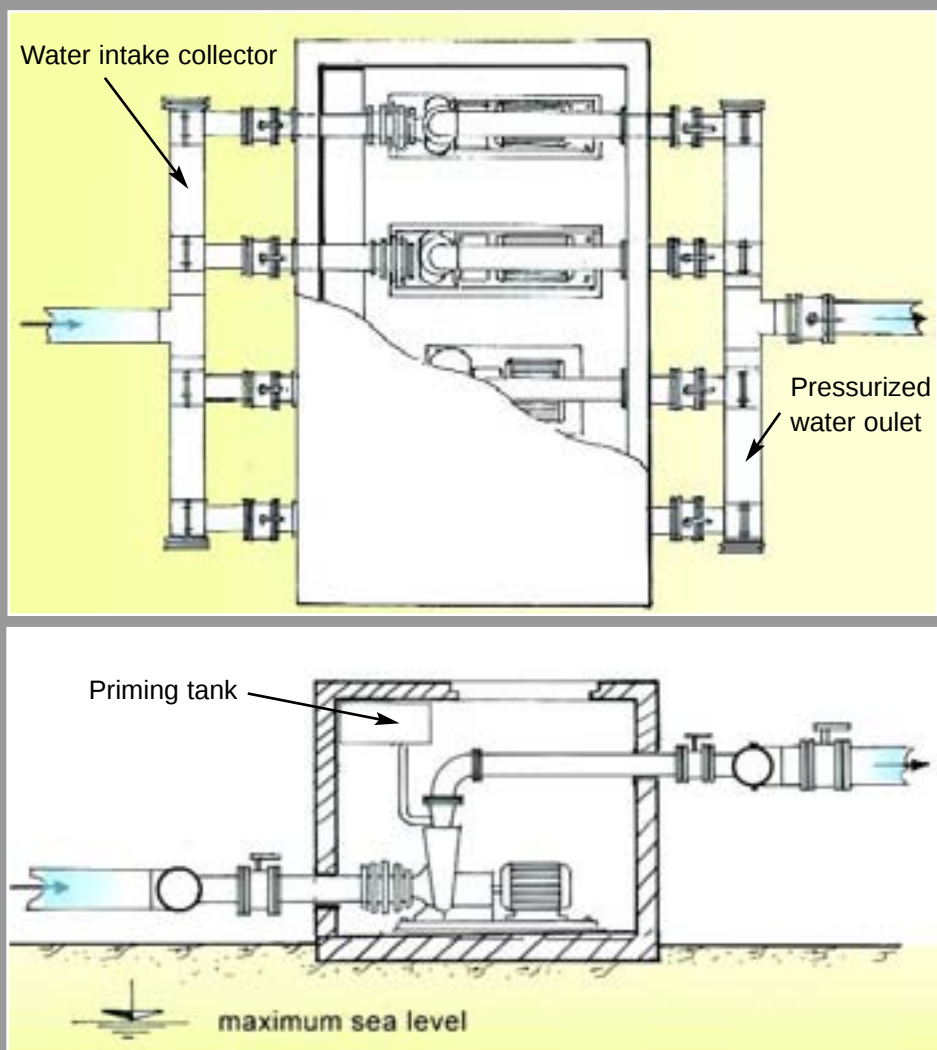
Fig. 45 - "Dry" pumping station. Top and lateral views
