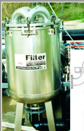
Fig. 62 - Bag filter
