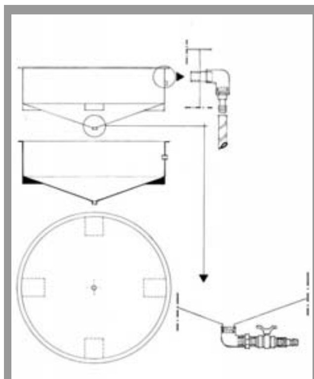
Fig. 19 - Fibreglass tank
