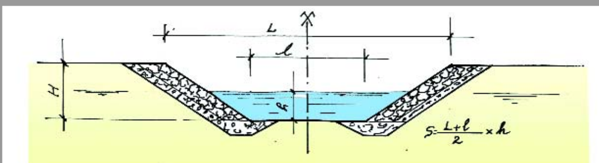
Fig. 42 - Open canal cross-section
