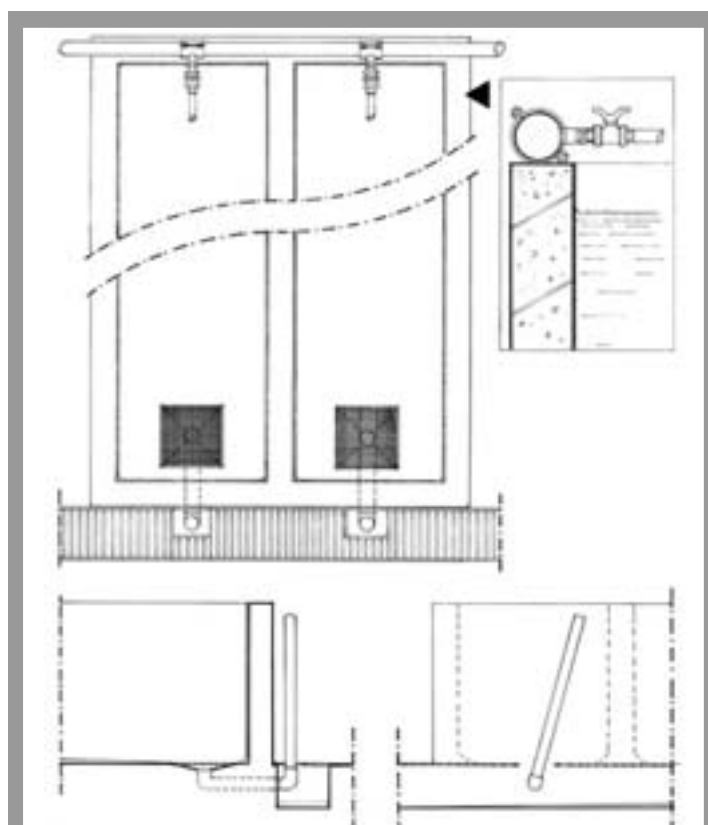
Fig. 23 - Concrete tanks
