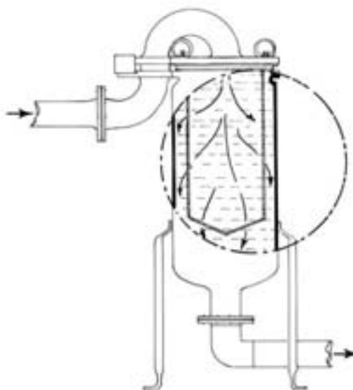
Fig. 59 - Mechanical filter
