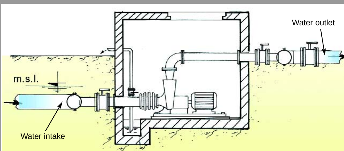
Fig . 46 - "Dry" pumping station below sea level
