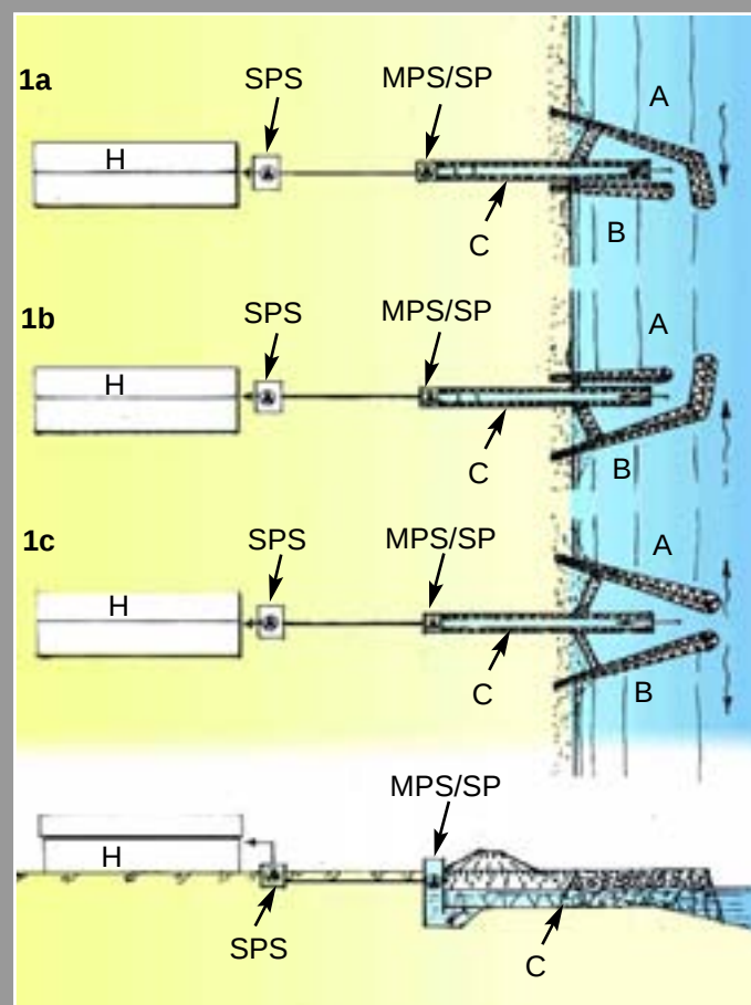
Fig. 29 - Water is pumped to a higher level at the end of the canal
