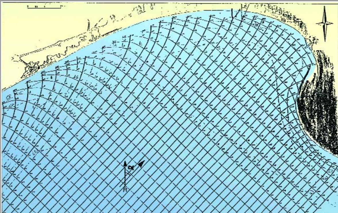
Fig. 39 - Wave spectrum and diffraction plans
