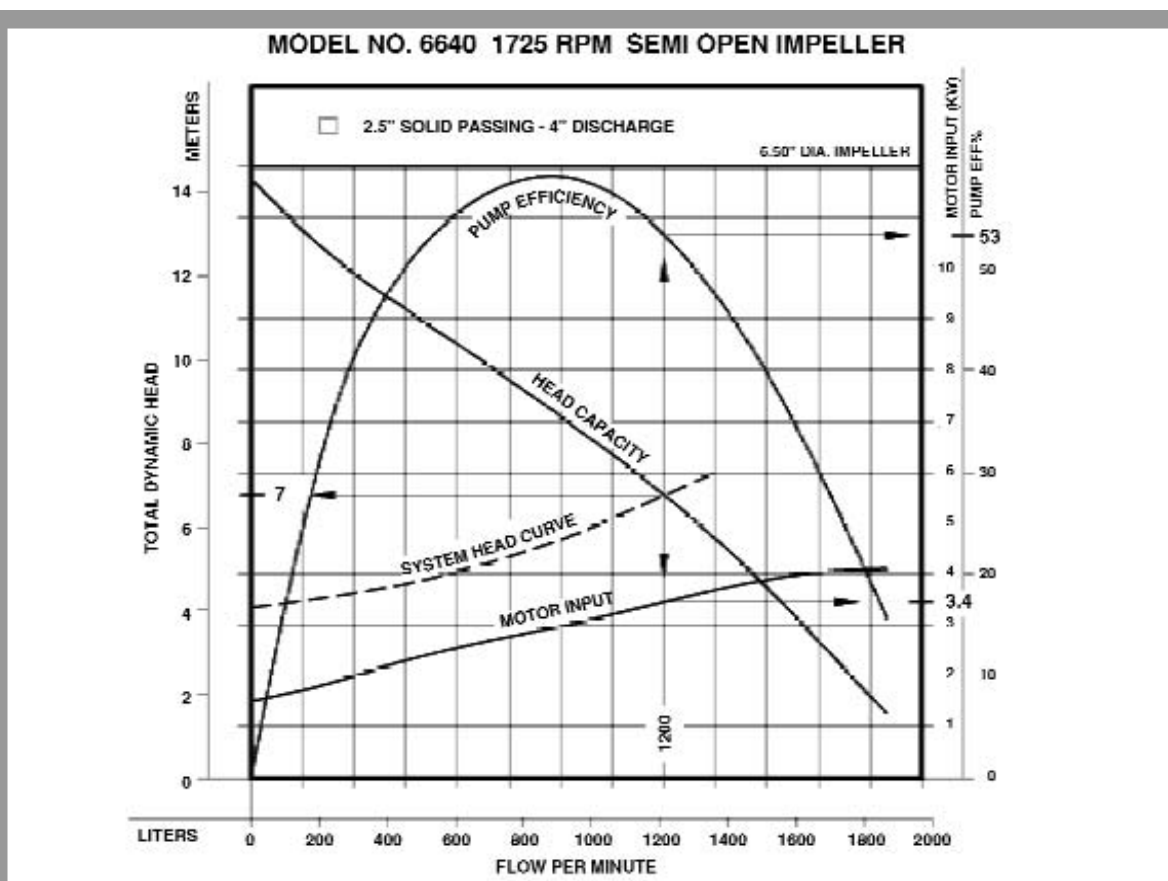
Fig. 56 - Typical pump curves (Source: J. Fletcher, Zoeller Company)
