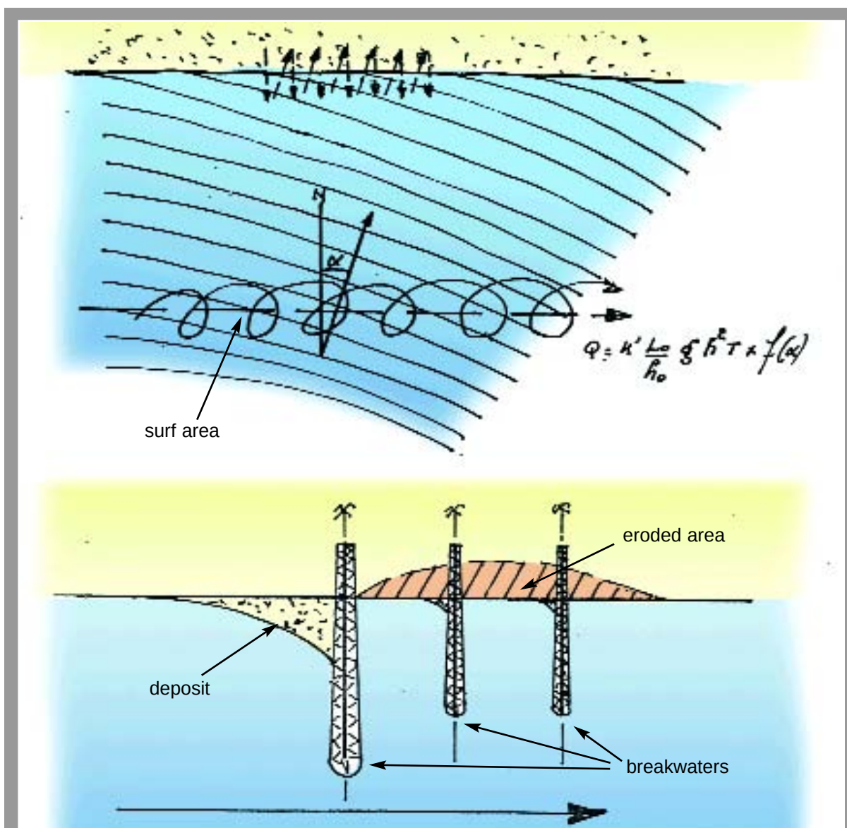
Fig. 38 - Sediment littoral transport by currents and waves. Effects of breakwaters on sediment transport
