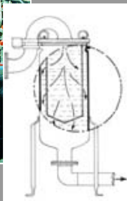
Fig. 62 - Bag filter
